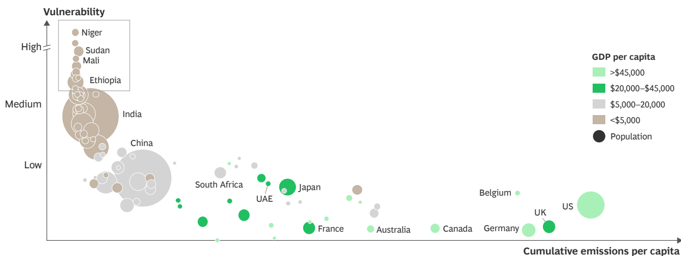
Cumulative CO 2 emissions vs. climate change vulnerability
