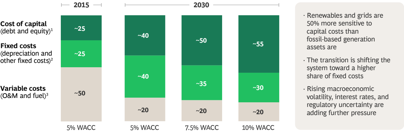
BREAKDOWN OF UK ELECTRICITY SYSTEM COSTS AT DIFFERENT WEIGHTED AVERAGE COSTS OF CAPITAL (%)
